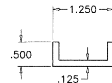
31 MOV. PANEL REINF.
