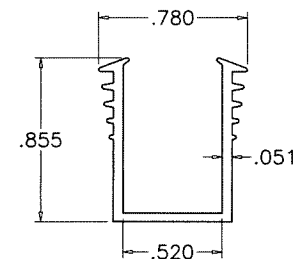
16 GLAZING GASKET SCALE 1:1
