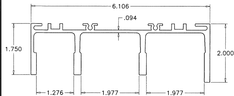
1A FRAME HEAD (WITHOUT SHEAR CLIPS)
